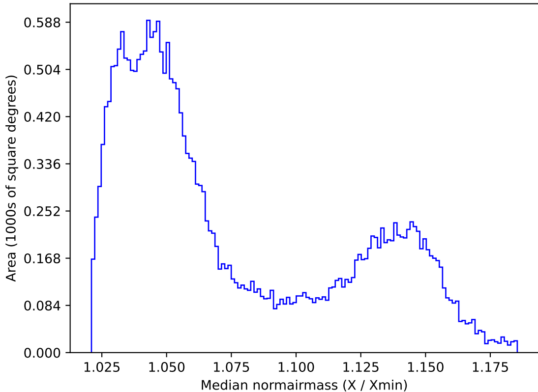
too_ignore_5_4v3.4_10yrs All sky all bands: Median normairmass
