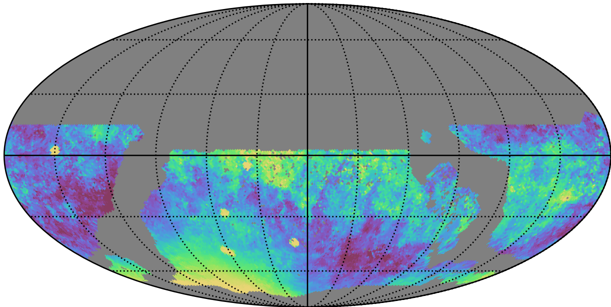
too_ignore_5_4v3.4_10yrs WFD z band: Median moonDistance
