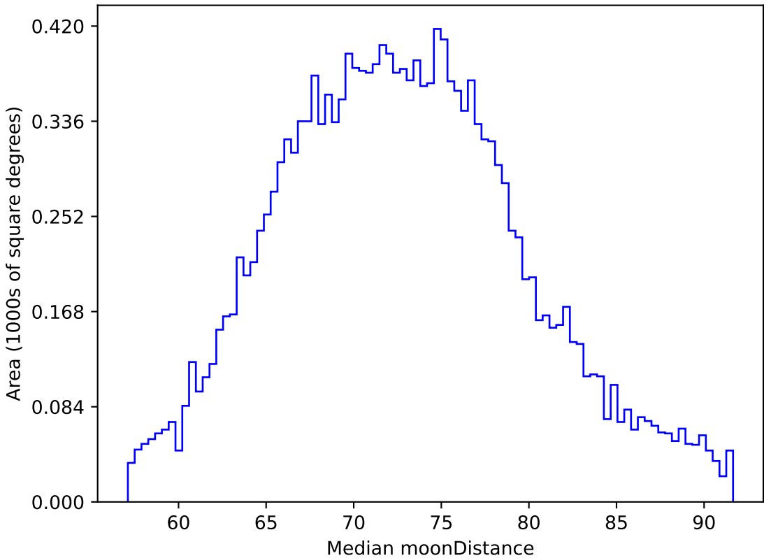
too_ignore_5_4v3.4_10yrs WFD z band: Median moonDistance
