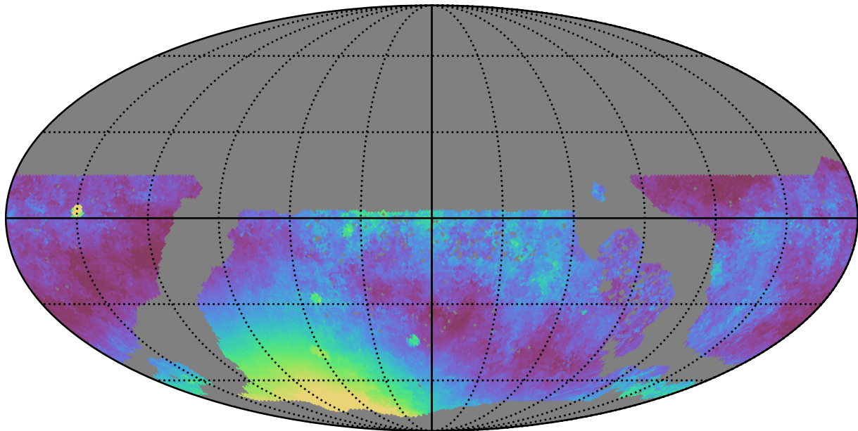
too_ignore_5_4v3.4_10yrs WFD y band: Median moonDistance
