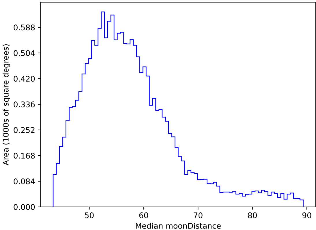
too_ignore_5_4v3.4_10yrs WFD y band: Median moonDistance
