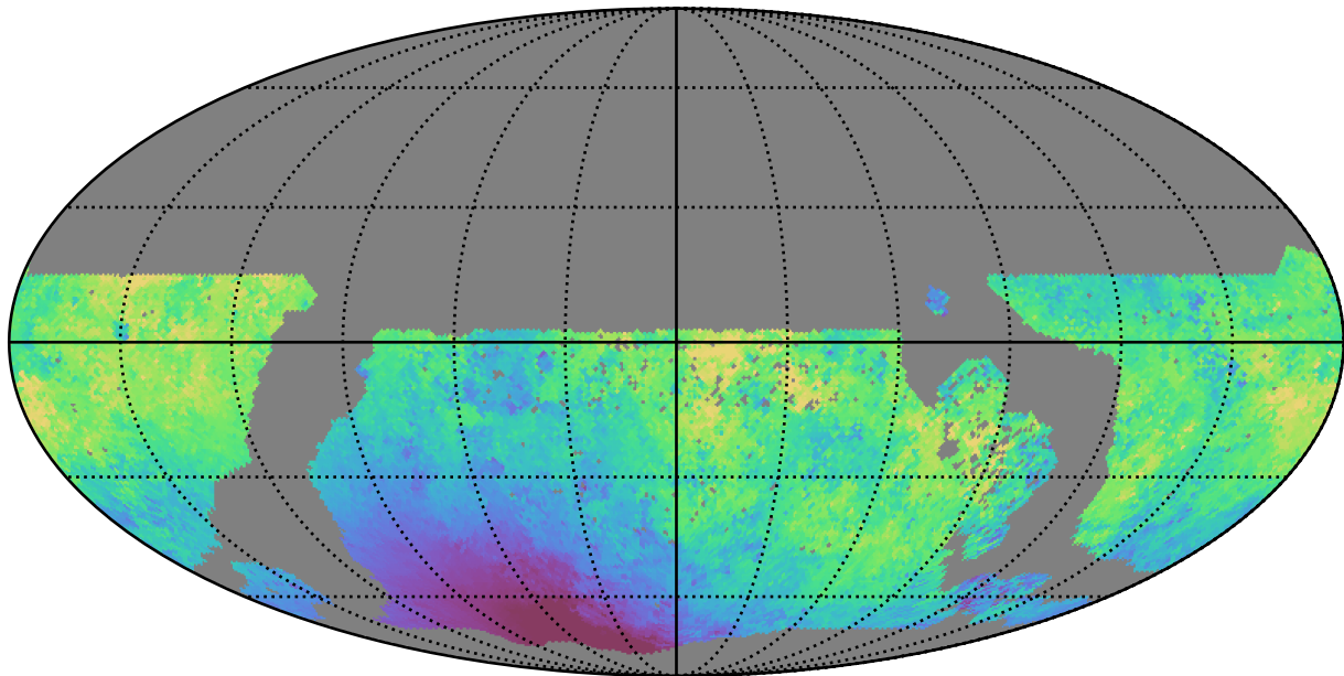
too_ignore_5_4v3.4_10yrs WFD u band: Median moonDistance
