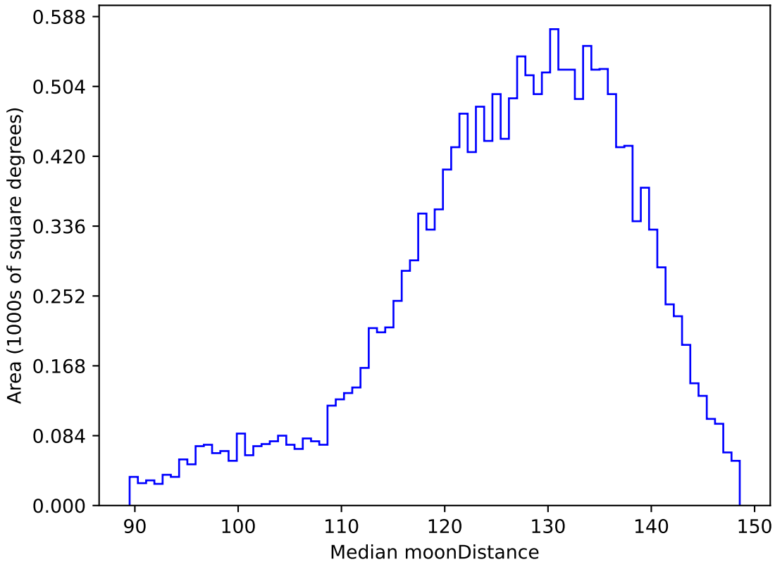
too_ignore_5_4v3.4_10yrs WFD u band: Median moonDistance
