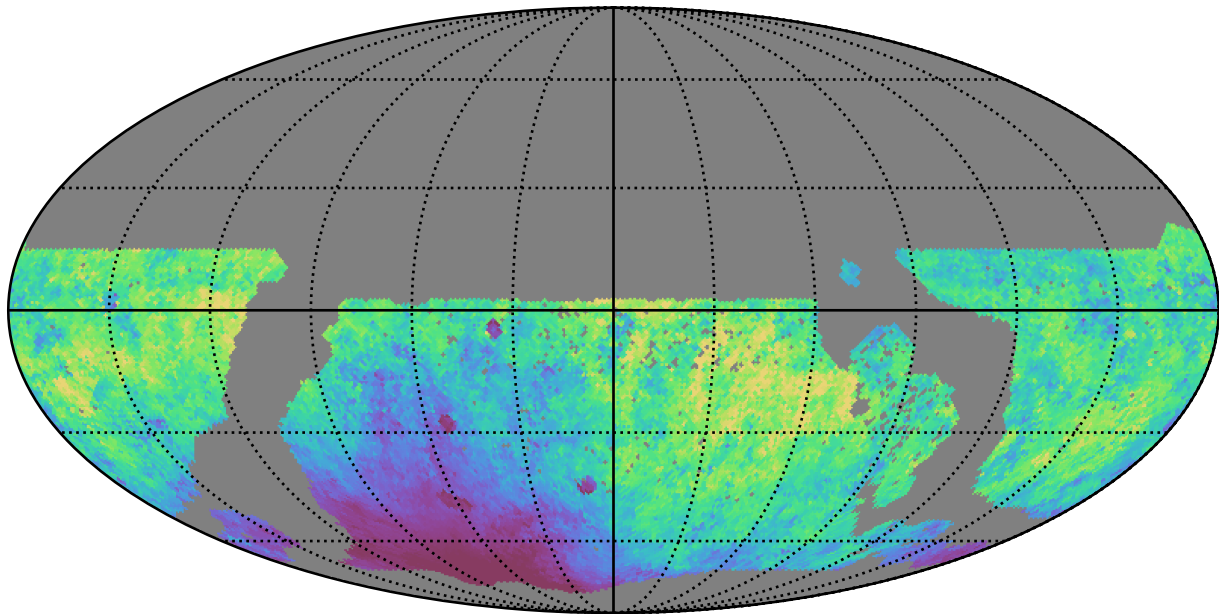
too_ignore_5_4v3.4_10yrs WFD r band: Median moonDistance
