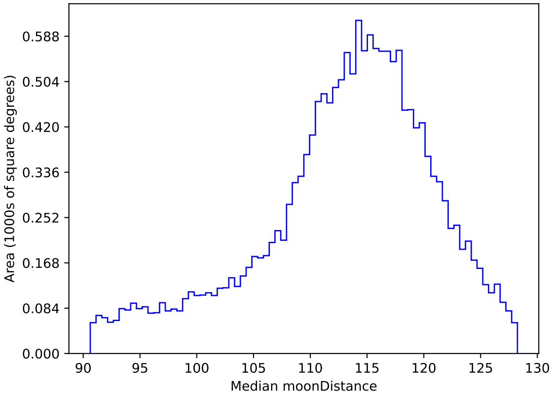
too_ignore_5_4v3.4_10yrs WFD r band: Median moonDistance
