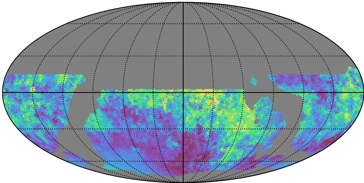
too_ignore_5_4v3.4_10yrs WFD i band: Median moonDistance
