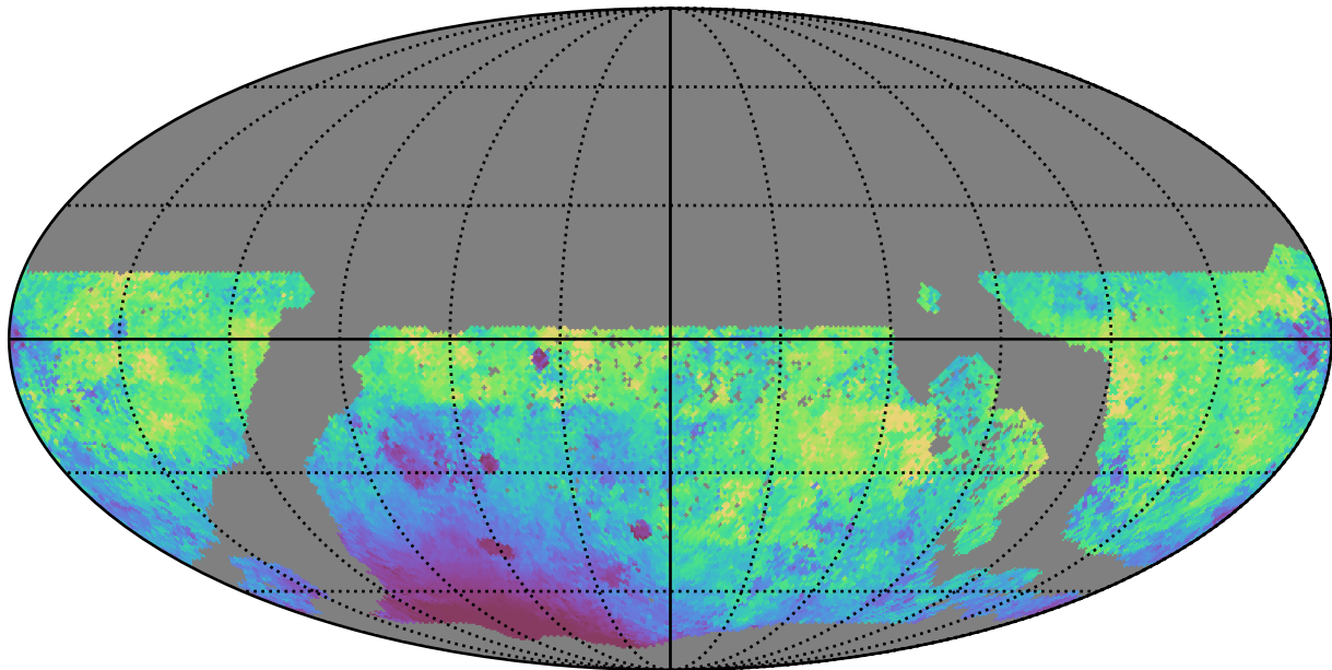
too_ignore_5_4v3.4_10yrs WFD g band: Median moonDistance
