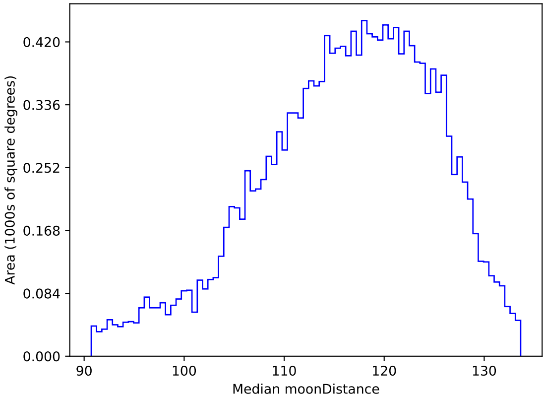
too_ignore_5_4v3.4_10yrs WFD g band: Median moonDistance
