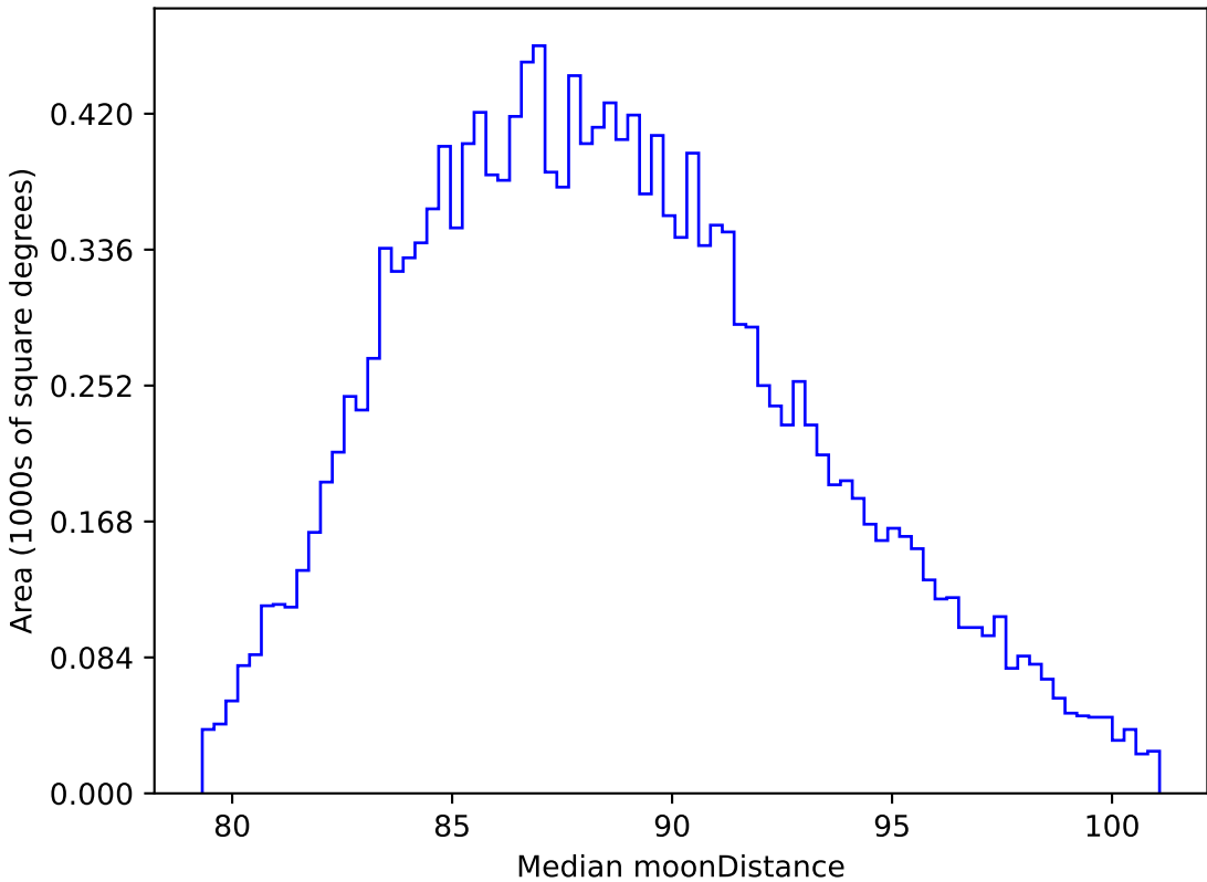
too_ignore_5_4v3.4_10yrs WFD all bands: Median moonDistance
