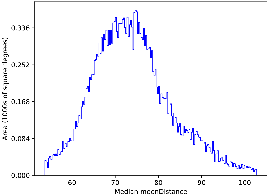
too_ignore_5_4v3.4_10yrs All sky z band: Median moonDistance
