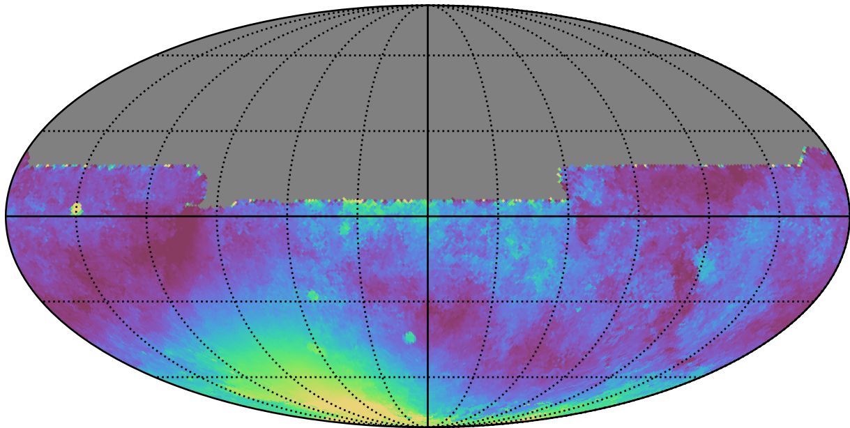
too_ignore_5_4v3.4_10yrs All sky y band: Median moonDistance
