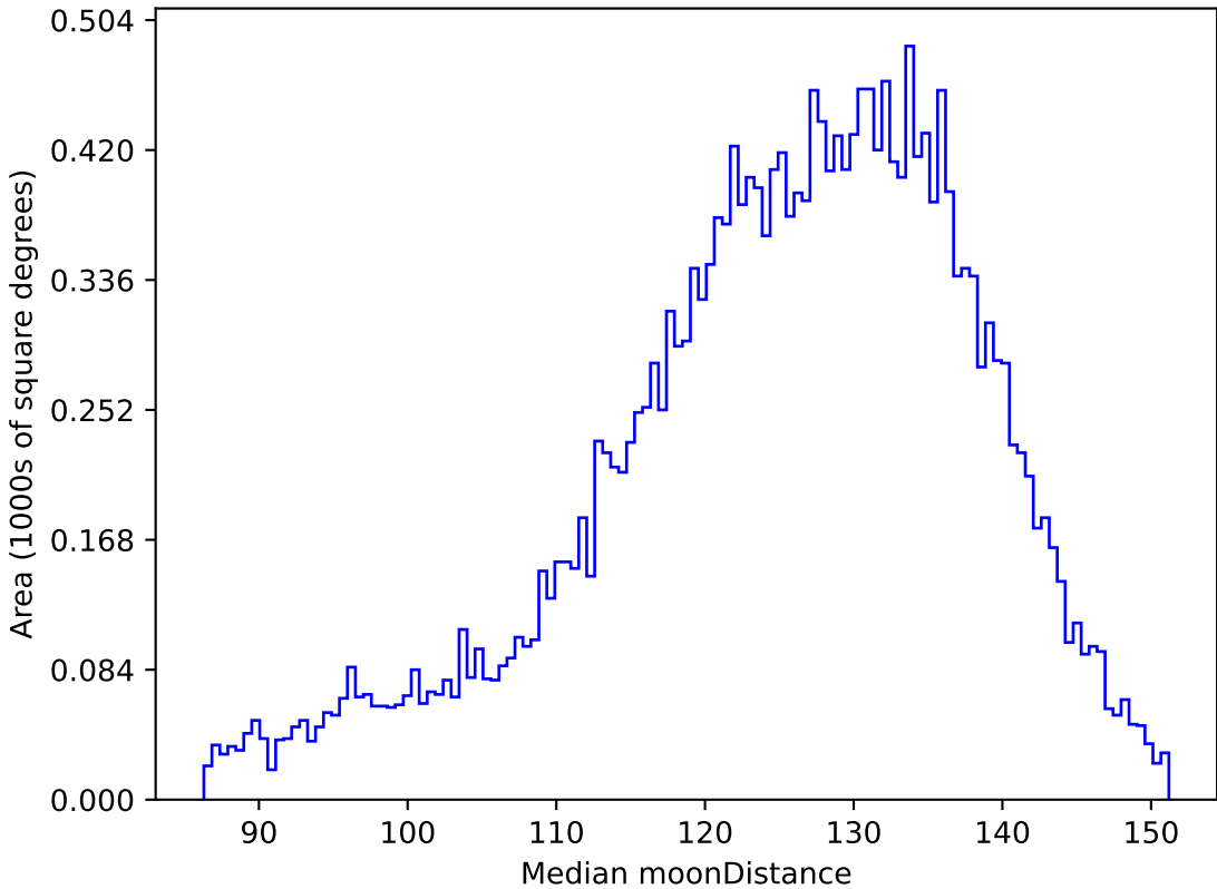
too_ignore_5_4v3.4_10yrs All sky u band: Median moonDistance
