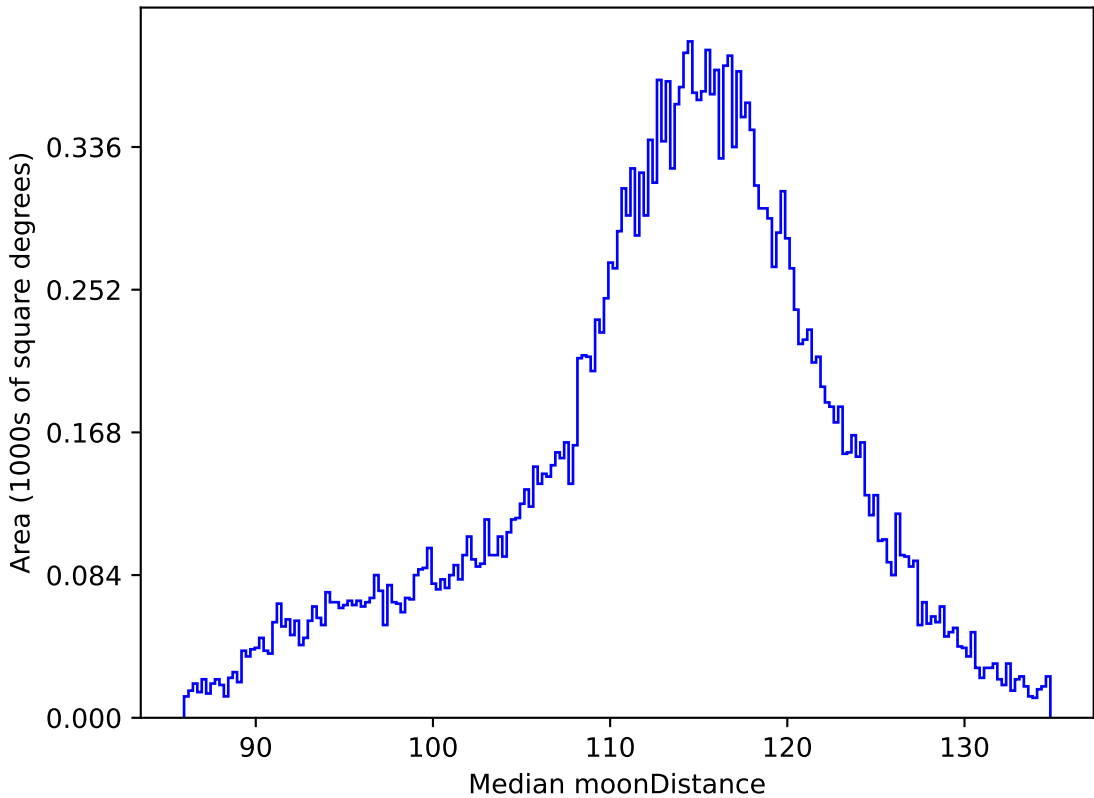
too_ignore_5_4v3.4_10yrs All sky r band: Median moonDistance
