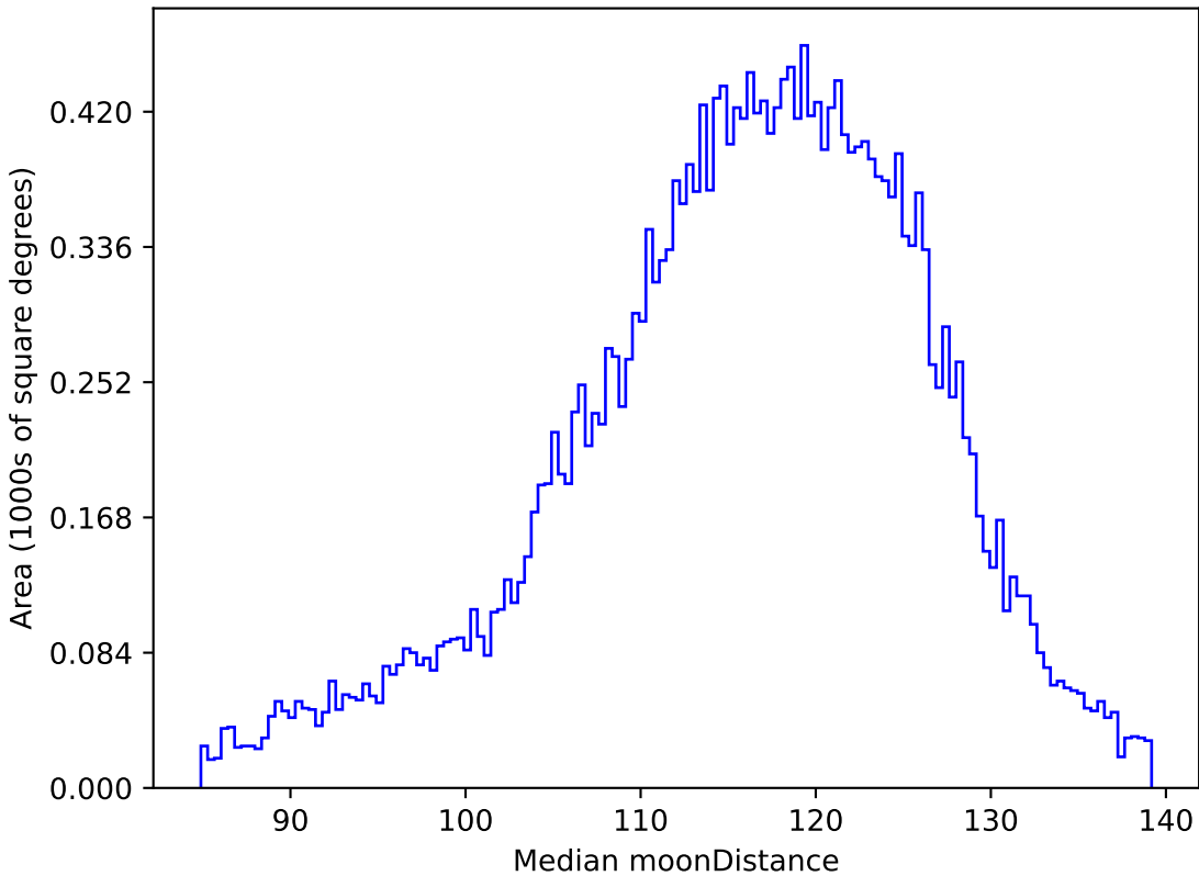
too_ignore_5_4v3.4_10yrs All sky g band: Median moonDistance
