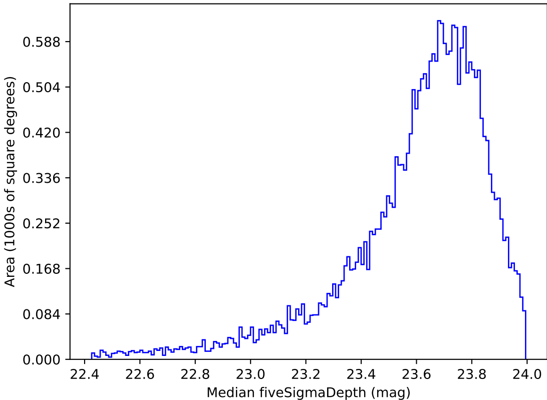
too_ignore_5_4v3.4_10yrs Yr 1 i band: Median fiveSigmaDepth
