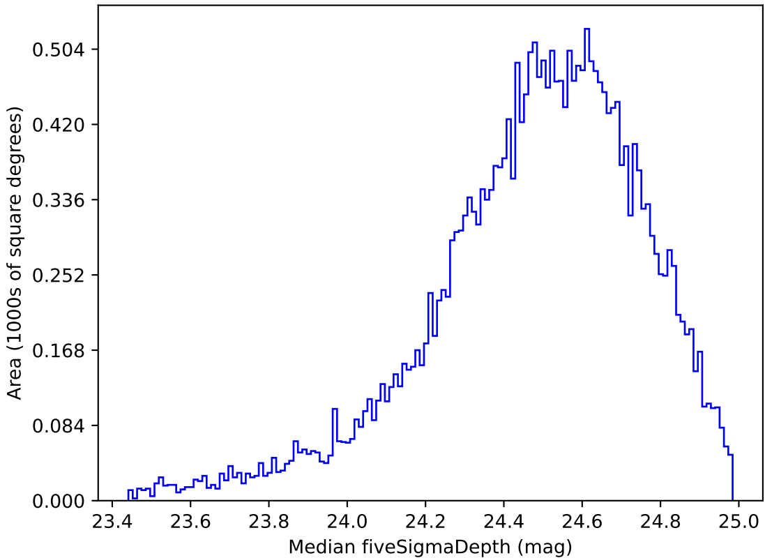
too_ignore_5_4v3.4_10yrs Yr 1 g band: Median fiveSigmaDepth
