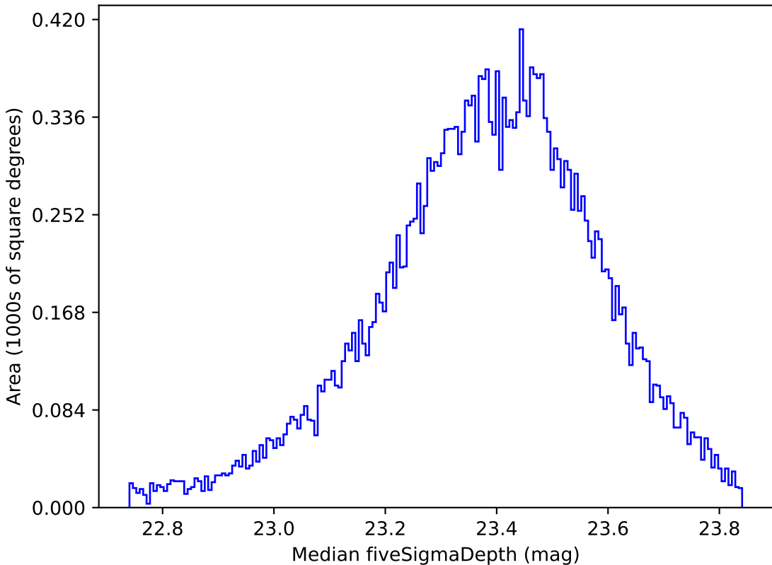
too_ignore_5_4v3.4_10yrs Yr 1 all bands: Median fiveSigmaDepth
