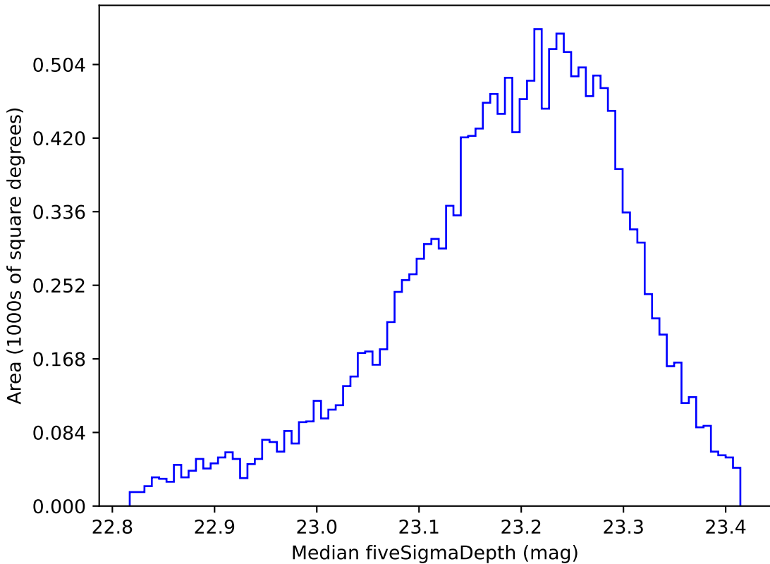
too_ignore_5_4v3.4_10yrs WFD u band: Median fiveSigmaDepth
