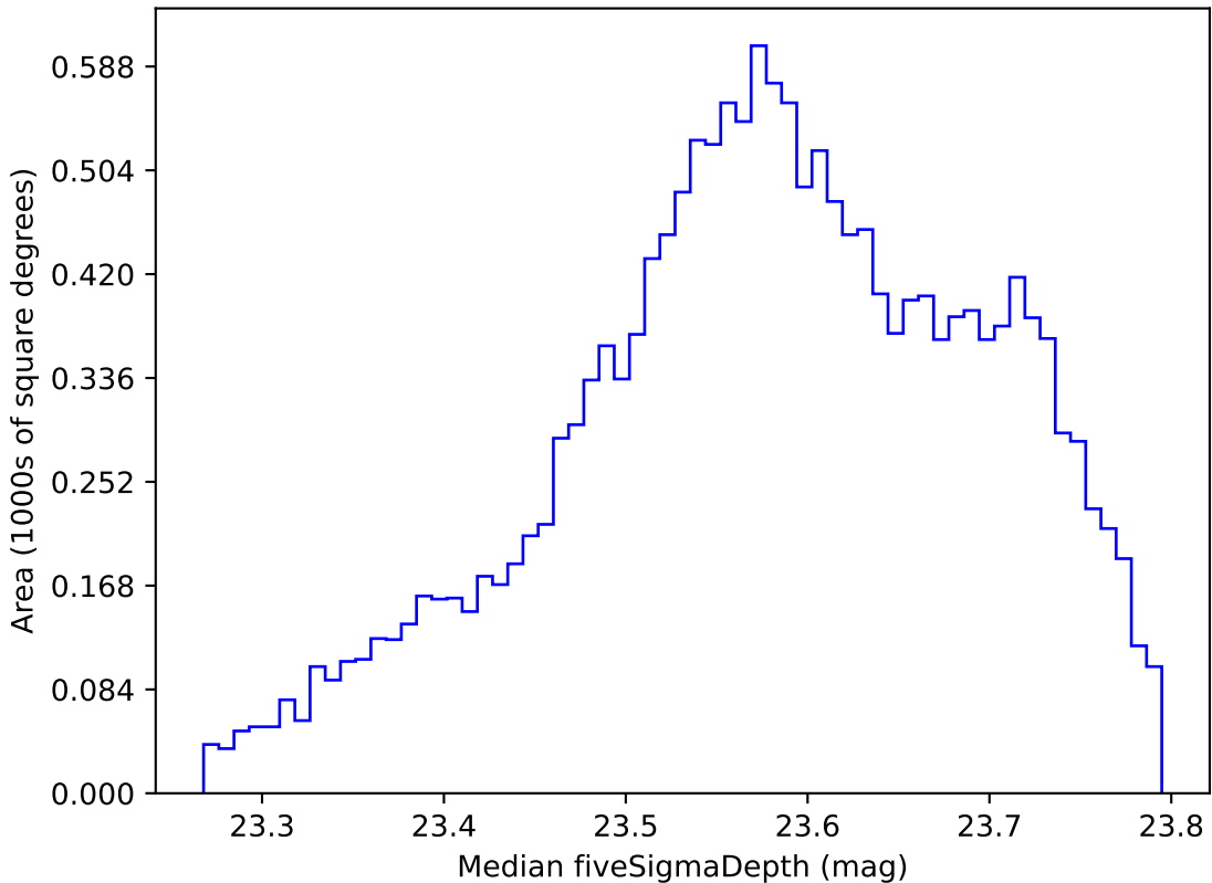
too_ignore_5_4v3.4_10yrs WFD i band: Median fiveSigmaDepth
