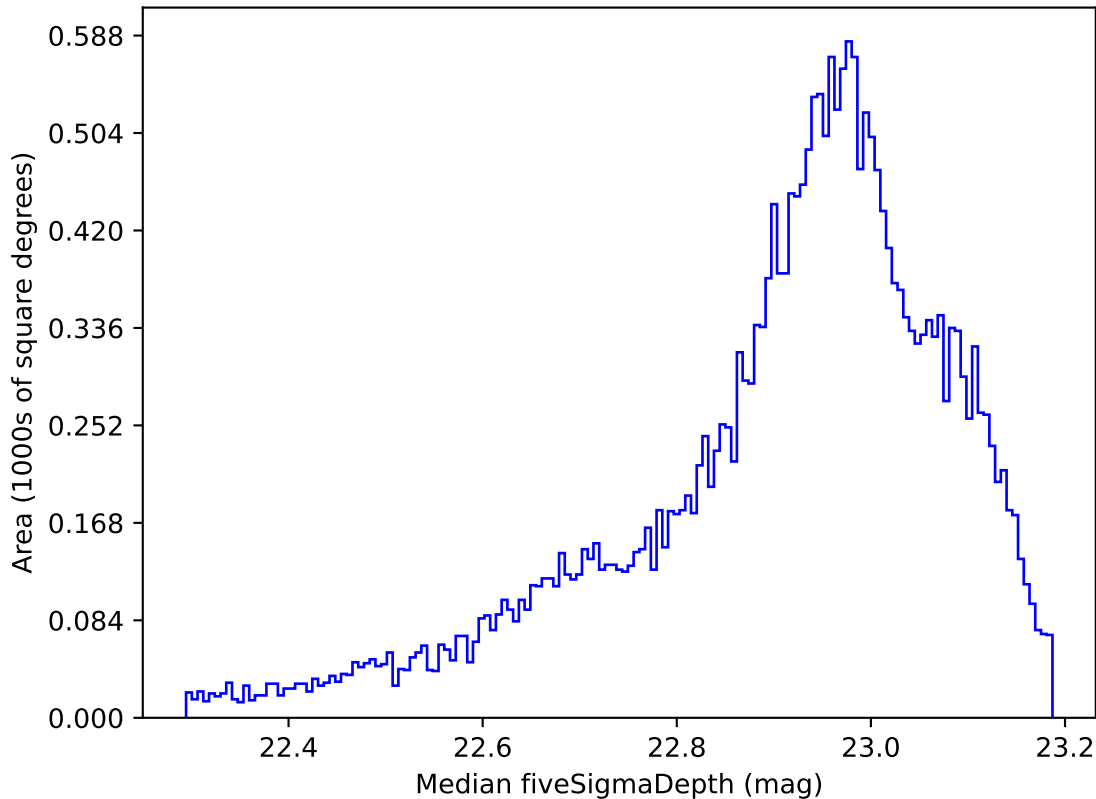
too_ignore_5_4v3.4_10yrs All sky z band: Median fiveSigmaDepth
