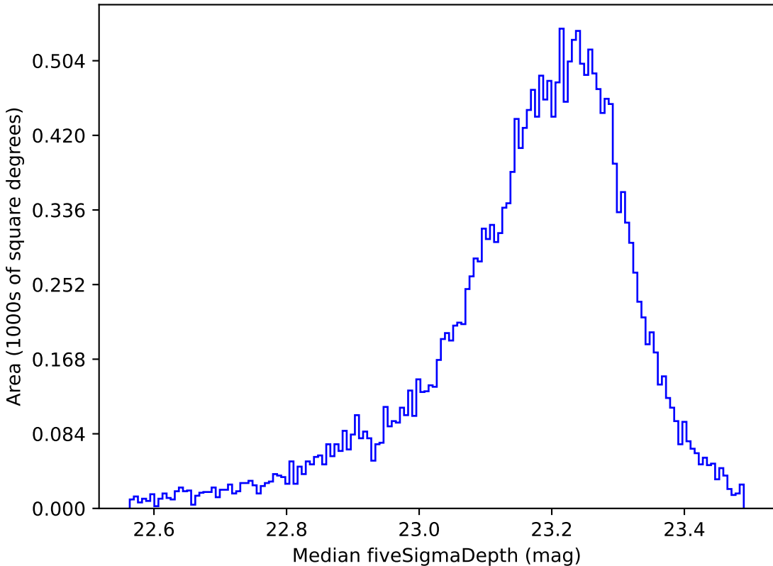
too_ignore_5_4v3.4_10yrs All sky u band: Median fiveSigmaDepth
