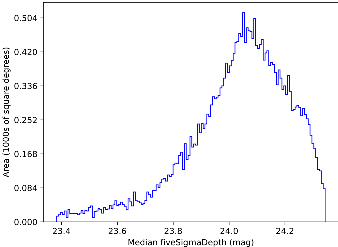
too_ignore_5_4v3.4_10yrs All sky r band: Median fiveSigmaDepth
