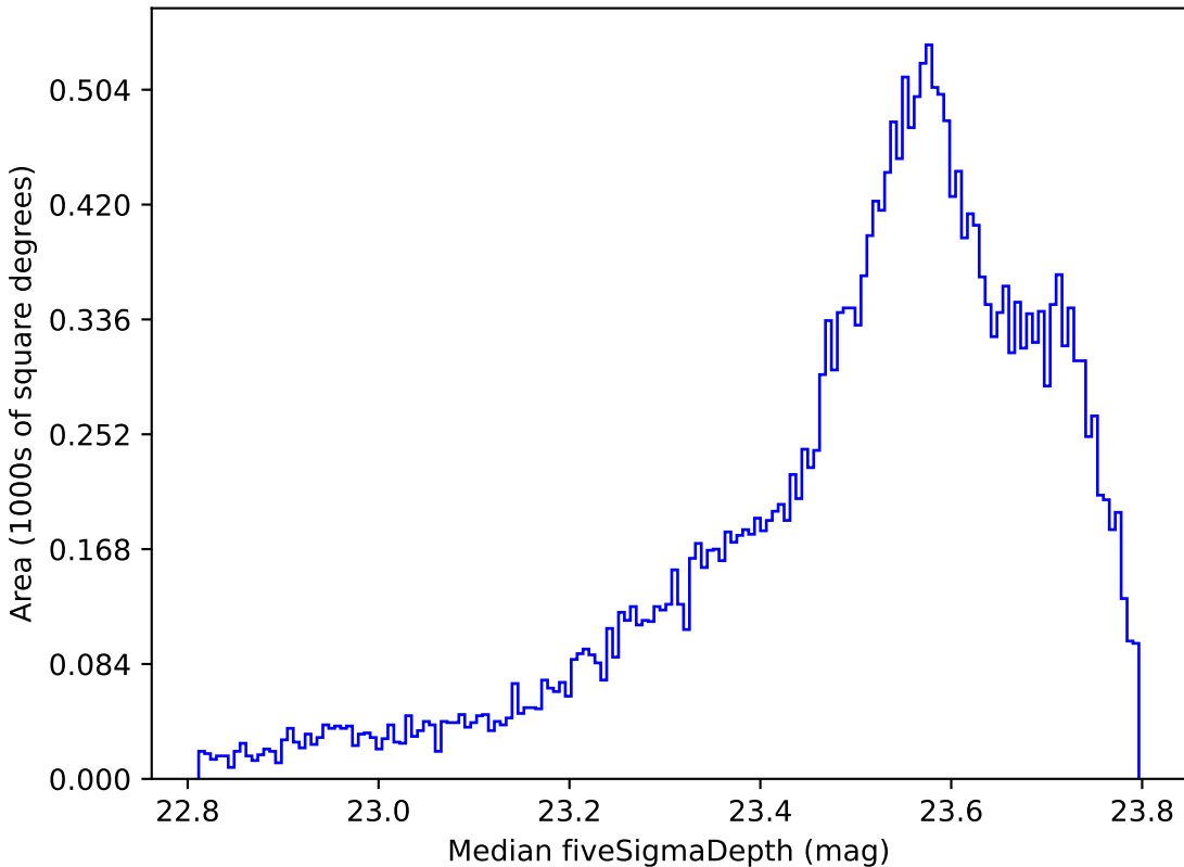
too_ignore_5_4v3.4_10yrs All sky i band: Median fiveSigmaDepth
