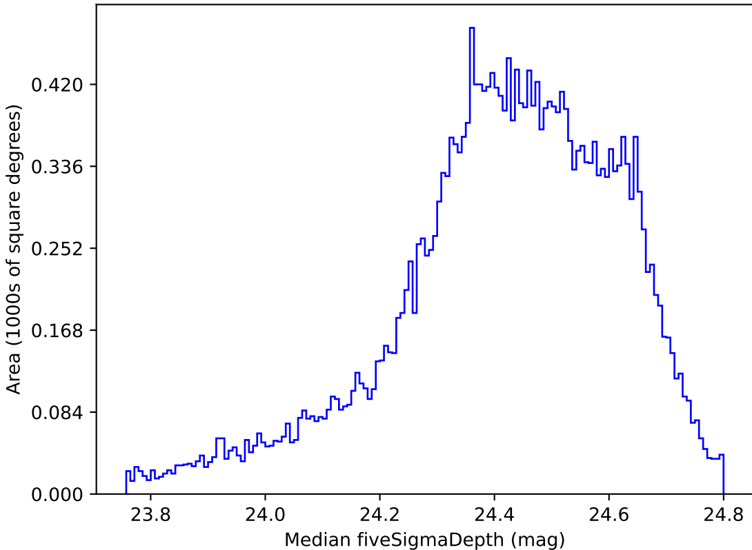
too_ignore_5_4v3.4_10yrs All sky g band: Median fiveSigmaDepth
