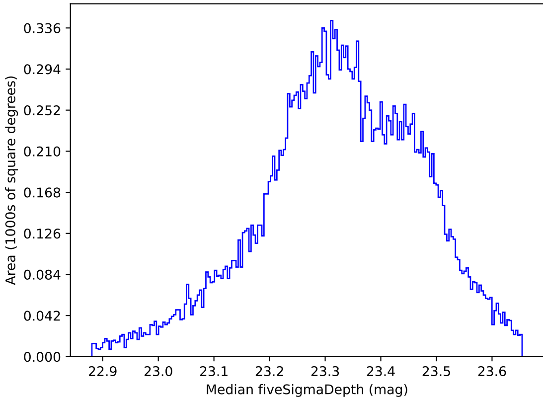
too_ignore_5_4v3.4_10yrs All sky all bands: Median fiveSigmaDepth
