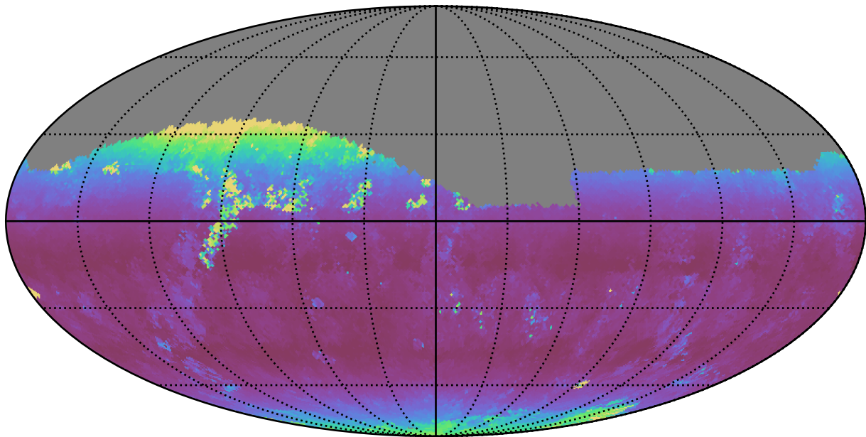
too_ignore_5_4v3.4_10yrs Yr 1 z band: Median airmass
