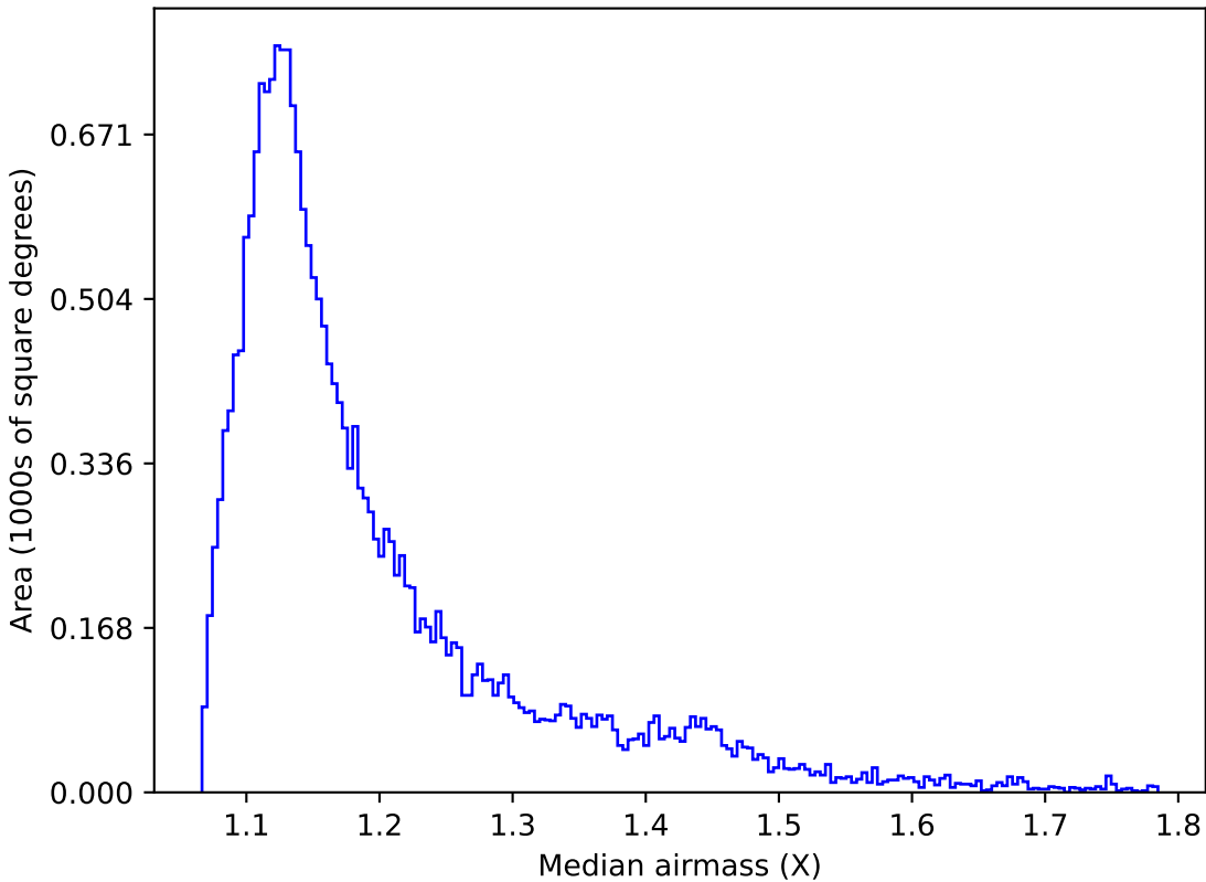
too_ignore_5_4v3.4_10yrs Yr 1 y band: Median airmass
