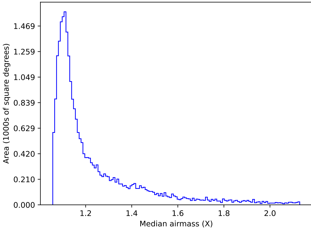
too_ignore_5_4v3.4_10yrs Yr 1 r band: Median airmass
