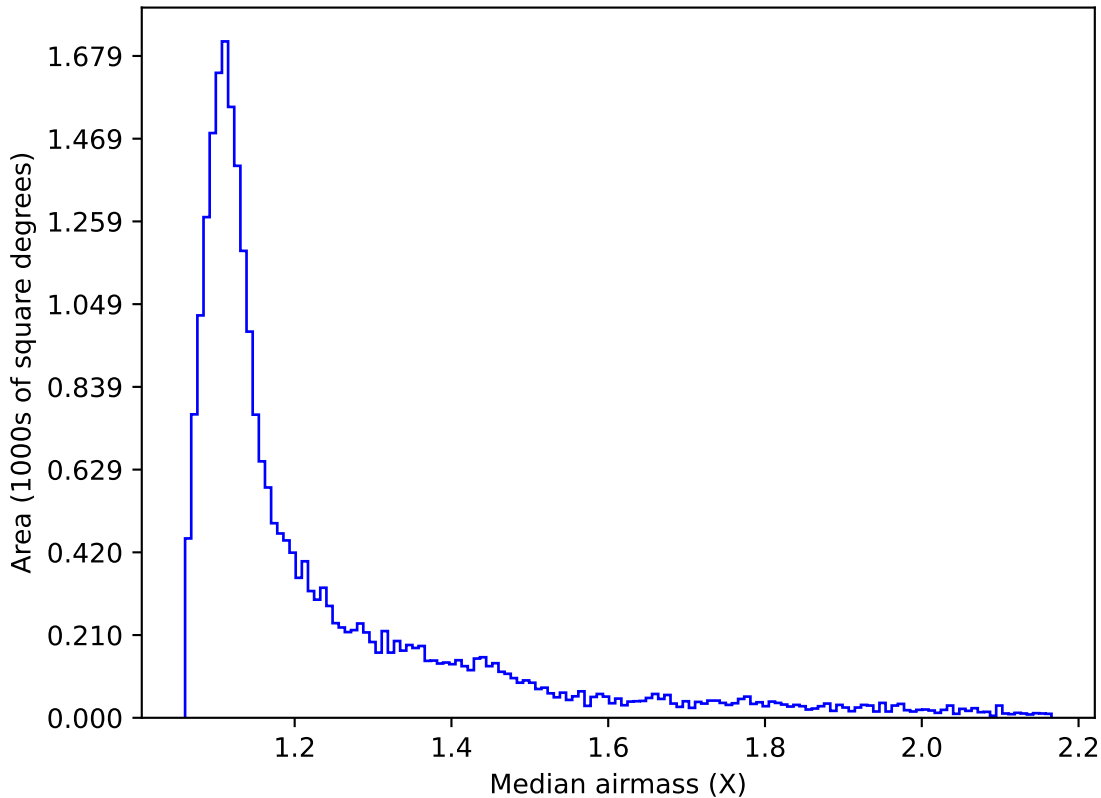
too_ignore_5_4v3.4_10yrs Yr 1 i band: Median airmass
