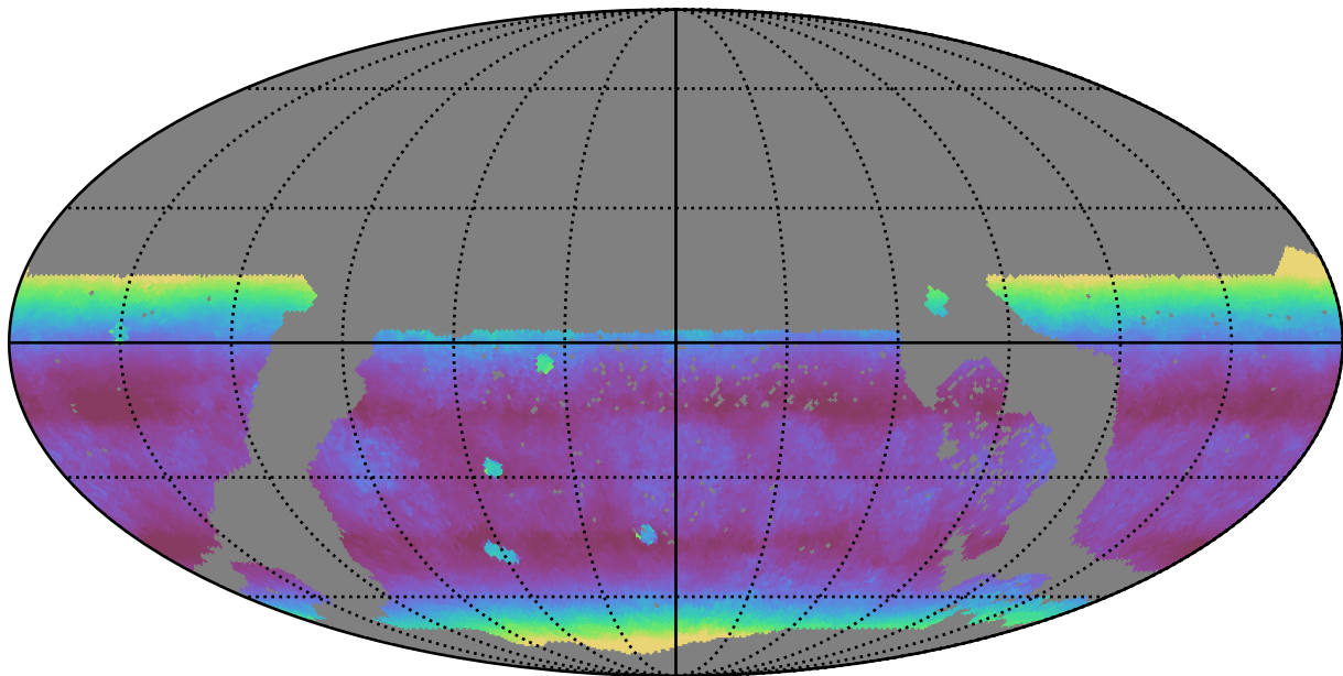
too_ignore_5_4v3.4_10yrs WFD z band: Median airmass
