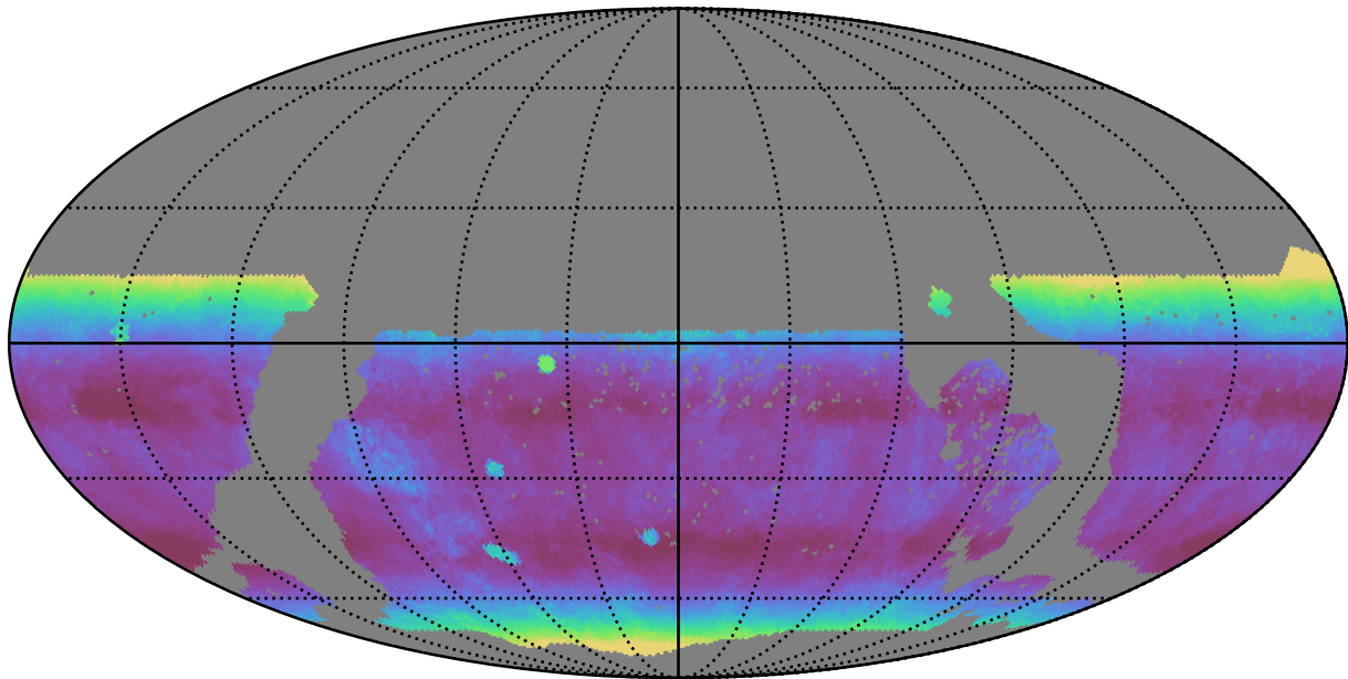
too_ignore_5_4v3.4_10yrs WFD y band: Median airmass
