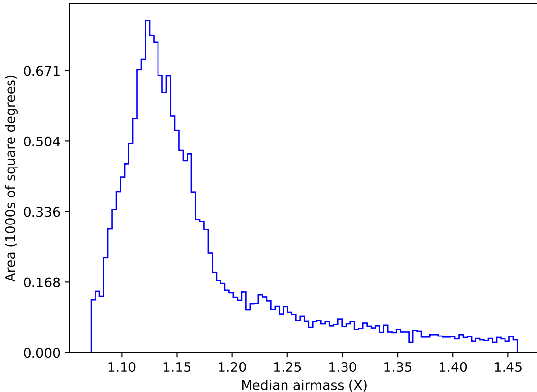
too_ignore_5_4v3.4_10yrs WFD r band: Median airmass
