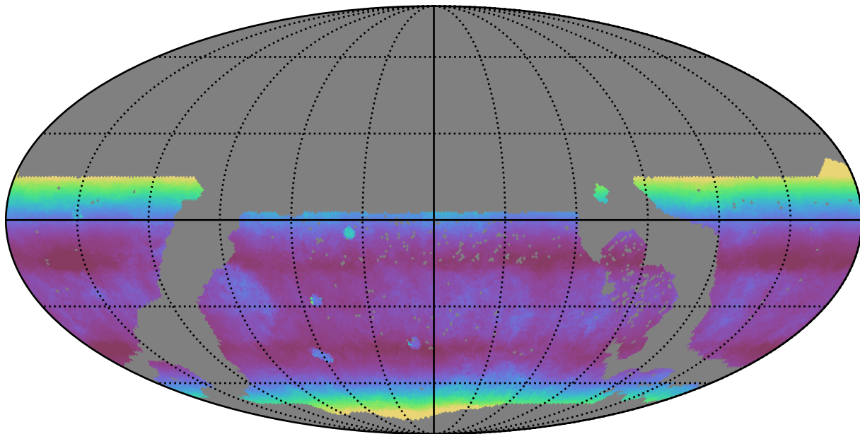
too_ignore_5_4v3.4_10yrs WFD i band: Median airmass
