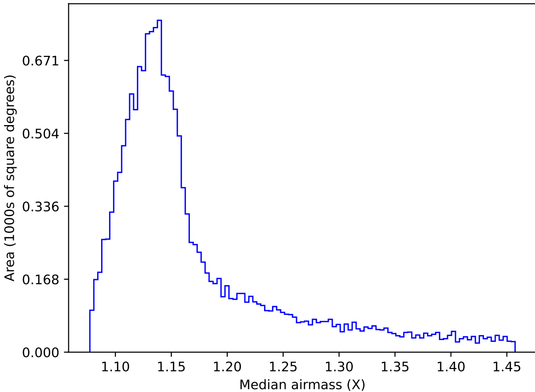
too_ignore_5_4v3.4_10yrs WFD i band: Median airmass
