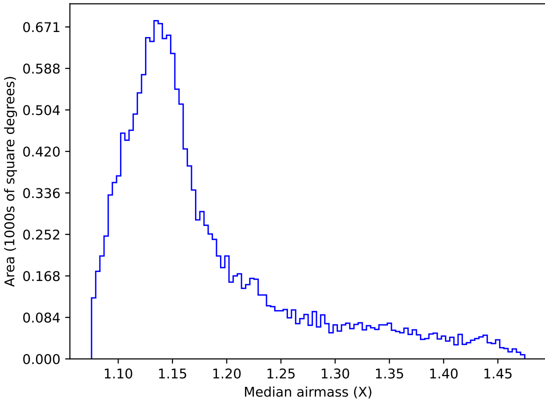
too_ignore_5_4v3.4_10yrs WFD g band: Median airmass
