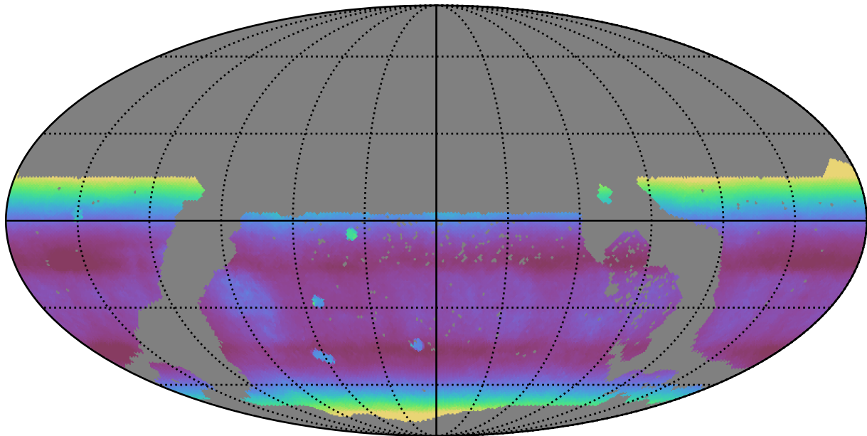
too_ignore_5_4v3.4_10yrs WFD all bands: Median airmass
