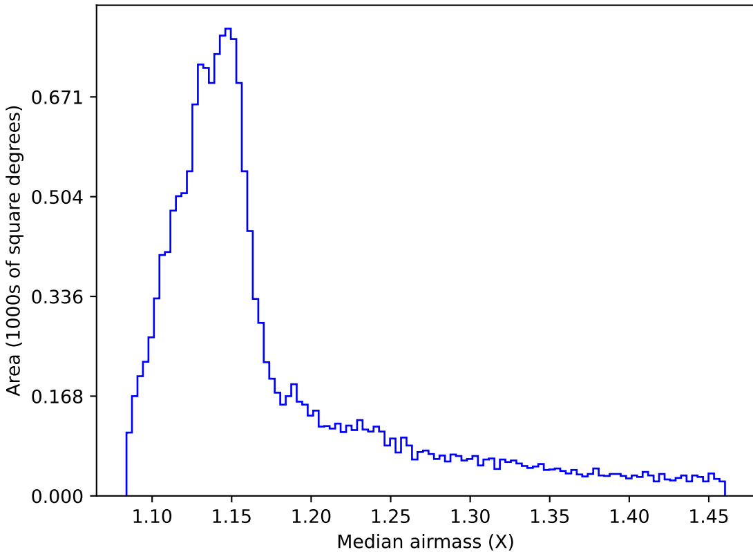
too_ignore_5_4v3.4_10yrs WFD all bands: Median airmass
