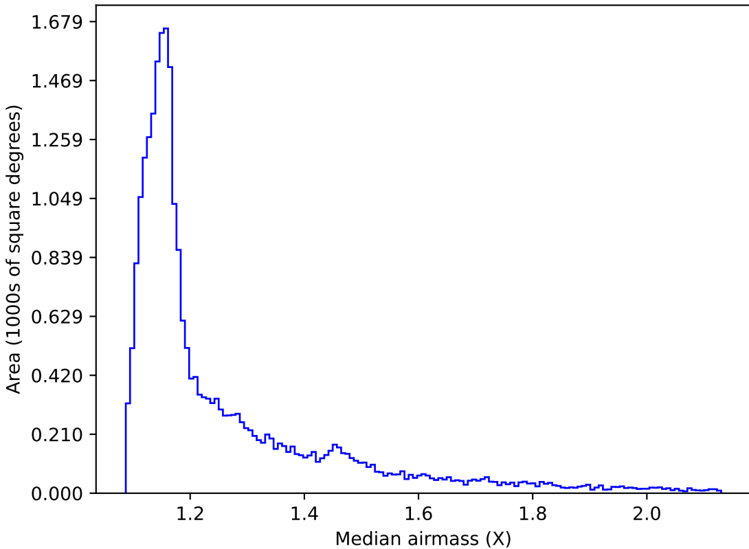
too_ignore_5_4v3.4_10yrs All sky z band: Median airmass
