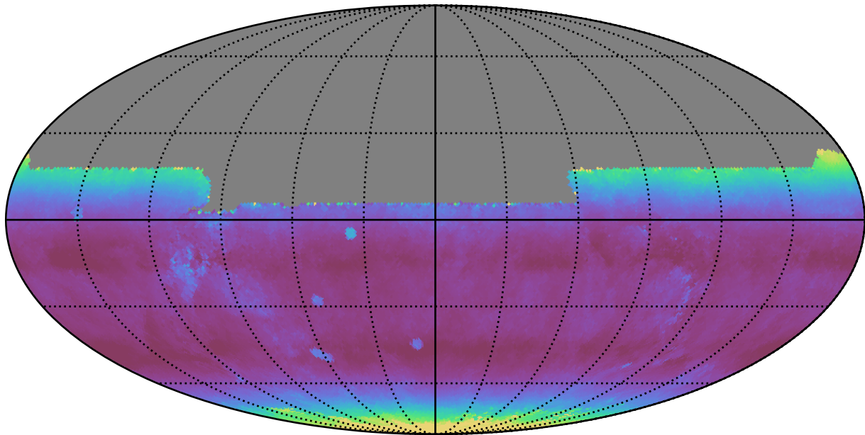
too_ignore_5_4v3.4_10yrs All sky y band: Median airmass
