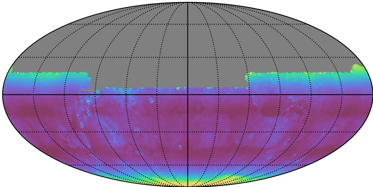
too_ignore_5_4v3.4_10yrs All sky u band: Median airmass
