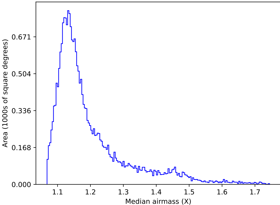
too_ignore_5_4v3.4_10yrs All sky u band: Median airmass
