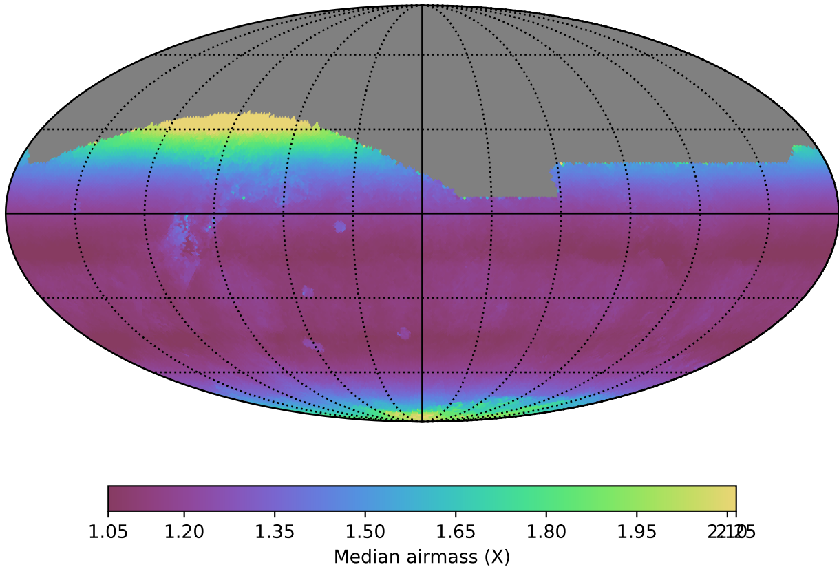
too_ignore_5_4v3.4_10yrs All sky r band: Median airmass
