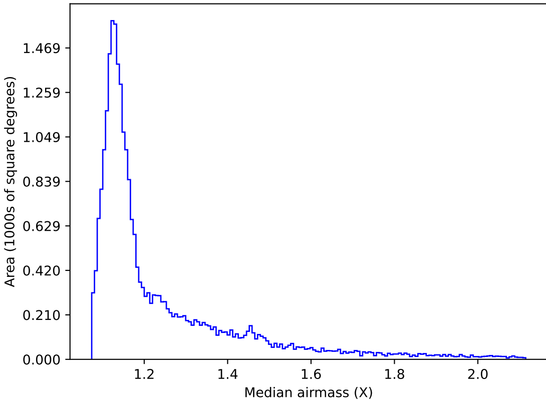
too_ignore_5_4v3.4_10yrs All sky r band: Median airmass
