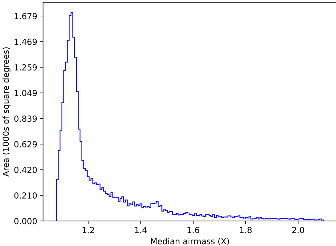
too_ignore_5_4v3.4_10yrs All sky i band: Median airmass
