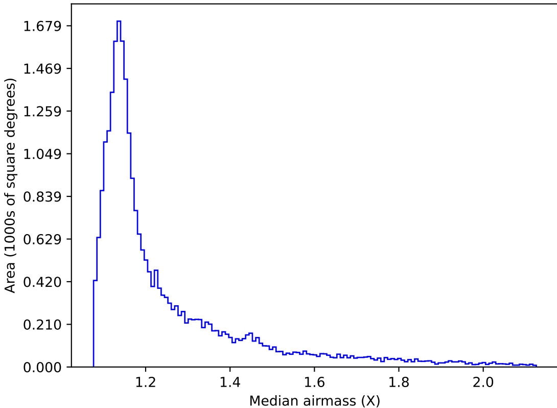
too_ignore_5_4v3.4_10yrs All sky g band: Median airmass
