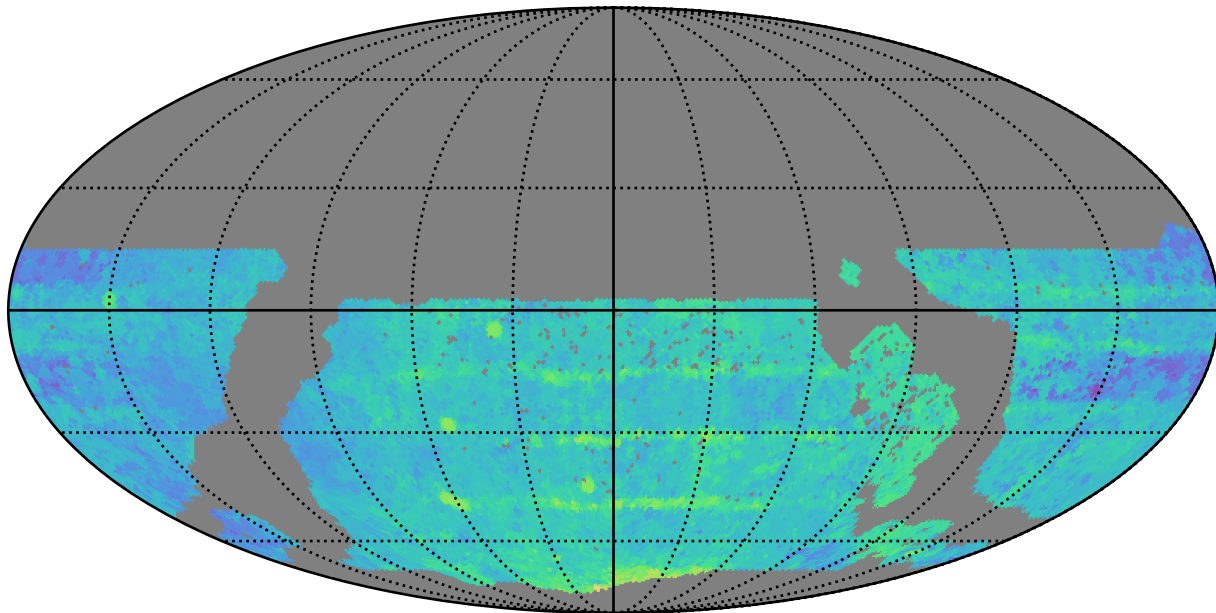
too_ignore_5_4v3.4_10yrs WFD z band: Median Season Length
